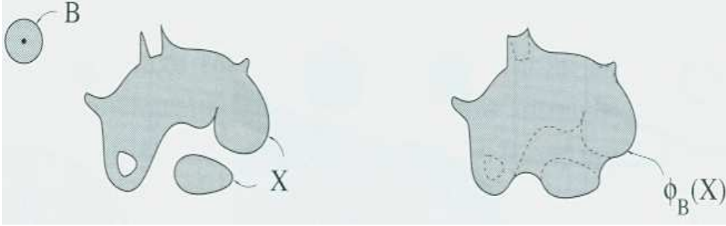
Figure 1: The effect of a closing operator on a non-smooth object (Reproduced from [42] with permission).
