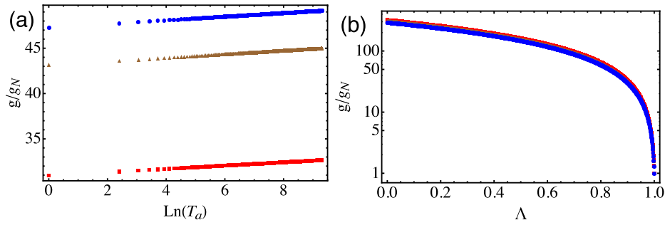
Figure 1: (Color online) Normalized cubic coefficient term, g/g_N , as a function of T_a (left) and \Lambda (right), for different values of M_1 . In both cases the fixed parameters are M_3 = 1.1 , P = 7 , \Gamma = 0.01 and a = 1 . Also, we have set in the left graph \Lambda = 0.9 and in the right graph T_a = 10 . The different values of M_1 are represented by different symbols M_1 = \{10, 5, 1\} = \{\blacksquare, \blacktriangle, \bullet\} .
